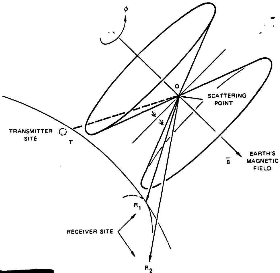
FIGURE 3-26. EQUIANGULAR SCATTERING GEOMETRY
